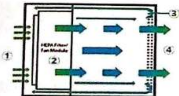
Horizontal Laminar flow Hood Diagram (Cutaway Side View)
