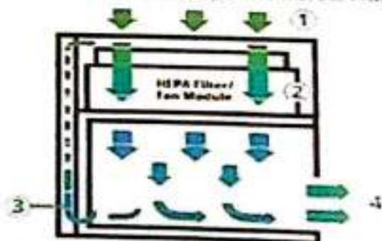
Vertical Laminar Flow Hood Diagram (Cutaway Side View)
