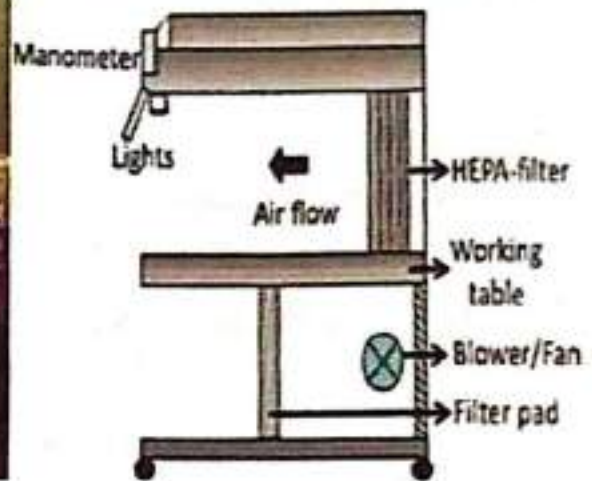
Horizontal Laminar Flow Cabinet
